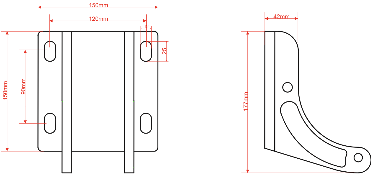
STANDARD BRACKET
