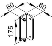
face fixture bracket assembly for the front profile 77822.
